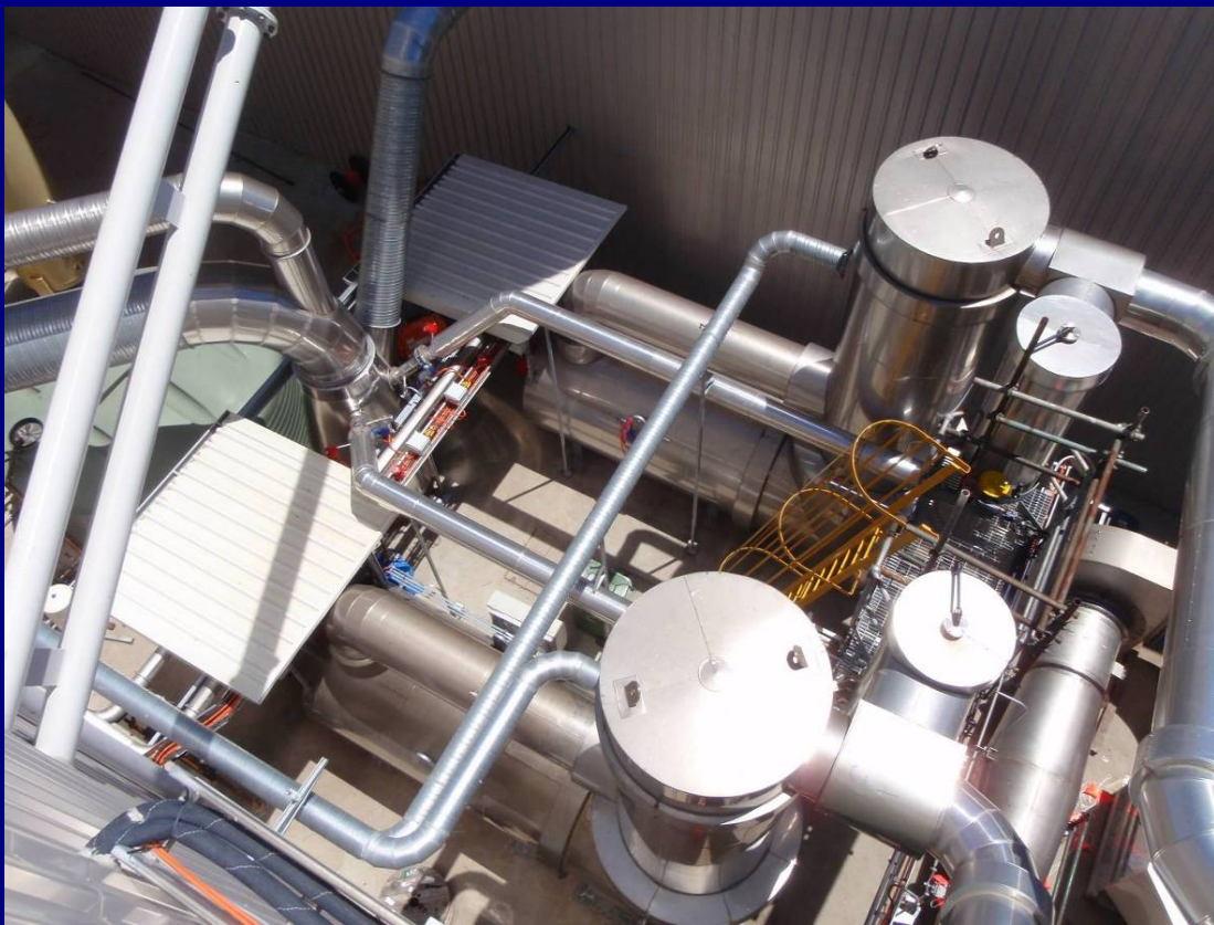
Process equipment installed and ready for commissioning.
